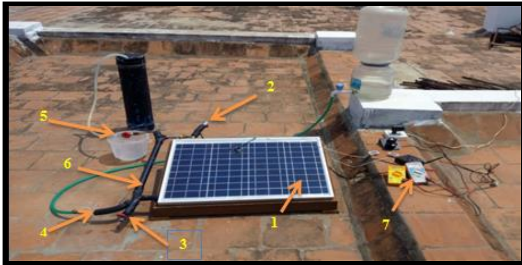
Fig 4. Experimental setup of PV/T systems with counter flow heat exchanger: (1) PV/T system, (2) nanofluid inlet, (3) nanofluid outlet, (4) water in, (5) hot water out, (6) counter flow heat exchanger and (7) instruments.
