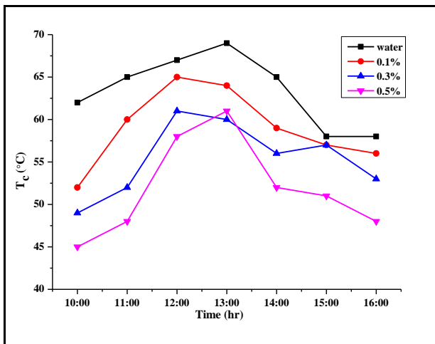
Fig 5. Cell surface temperature vs time
