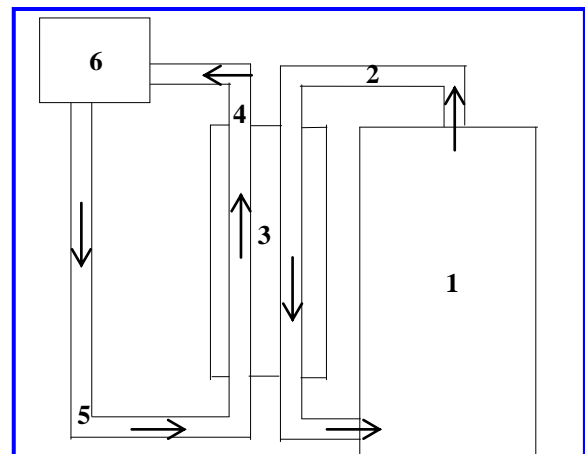
Fig 2. Line sketch of PV/T system with closed loop spiral flow arrangement and counter flow heat exchanger. (1) PV/T system, (2) nanofluid loop, (3) counter flow heat exchanger, (4) hot water outlet, (5) water inlet and (6) storage tank.
