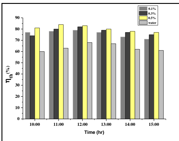
Fig 6. Thermal efficiency vs time
