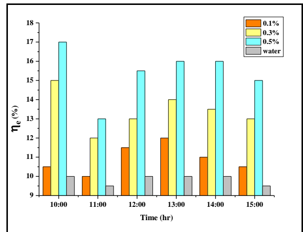
Fig 7. Electrical efficiency vs time
